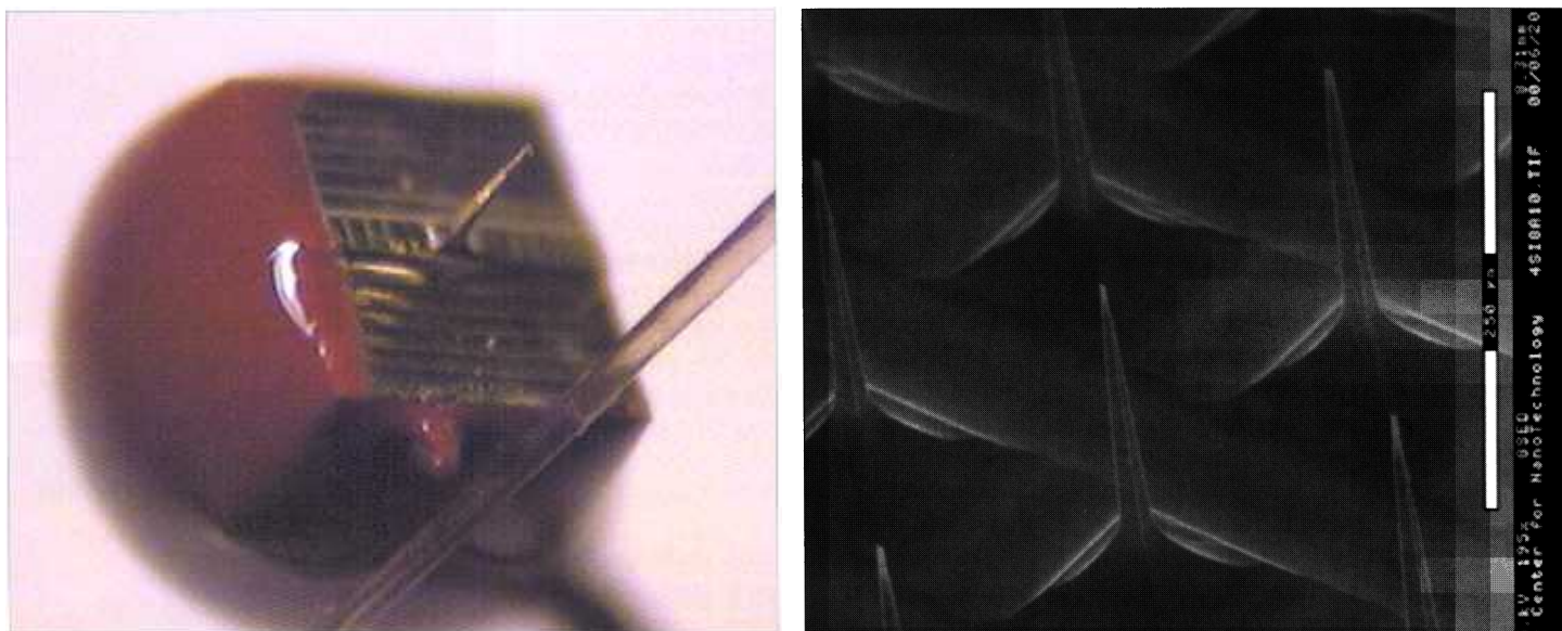
(Left) A prototype microchip with a silicon electrode to record the inner workings of Tritonia brain cells. A human hair is shown for scale. (Right) Future chips will contain a whole array of tiny silicon electrodes.
